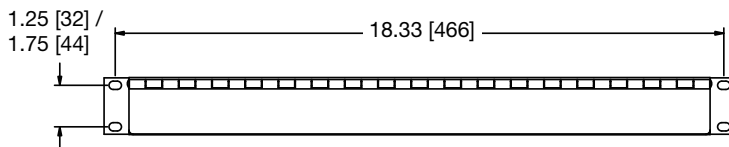
FRONT VIEW
